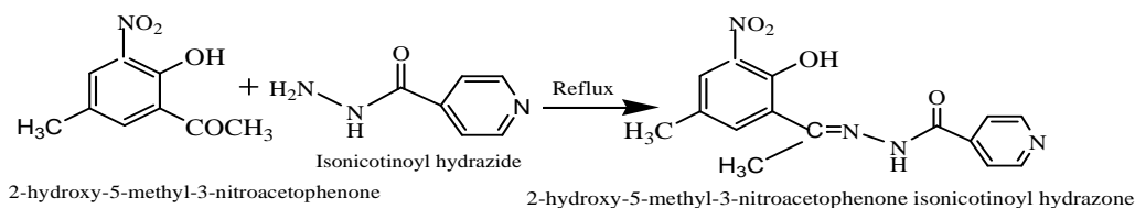
Scheme 1-Synthesis of the ligand (LH 2 )
