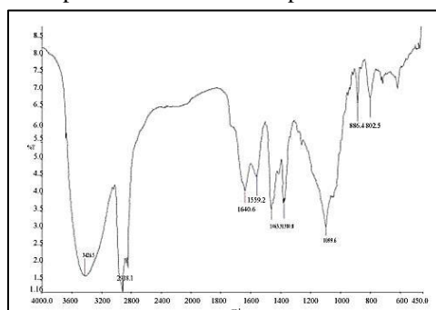
Figure 2: Spectrum IR of isolate
