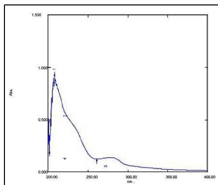
Figure 1: Spectrum UV-Vis for the isolate of derris plant
