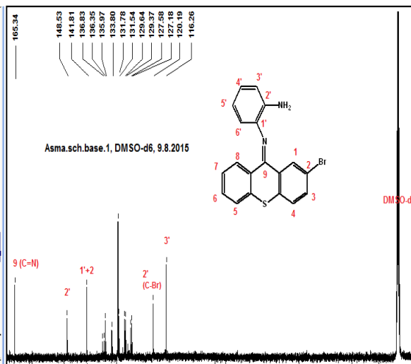
Figure (2): ¹³C-NMR spectrum for compound (11)
