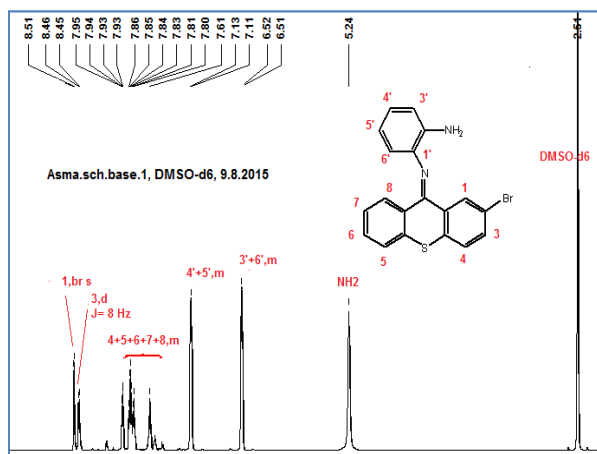
Figure (3): ¹H-NMR spectrum for compound (11)
