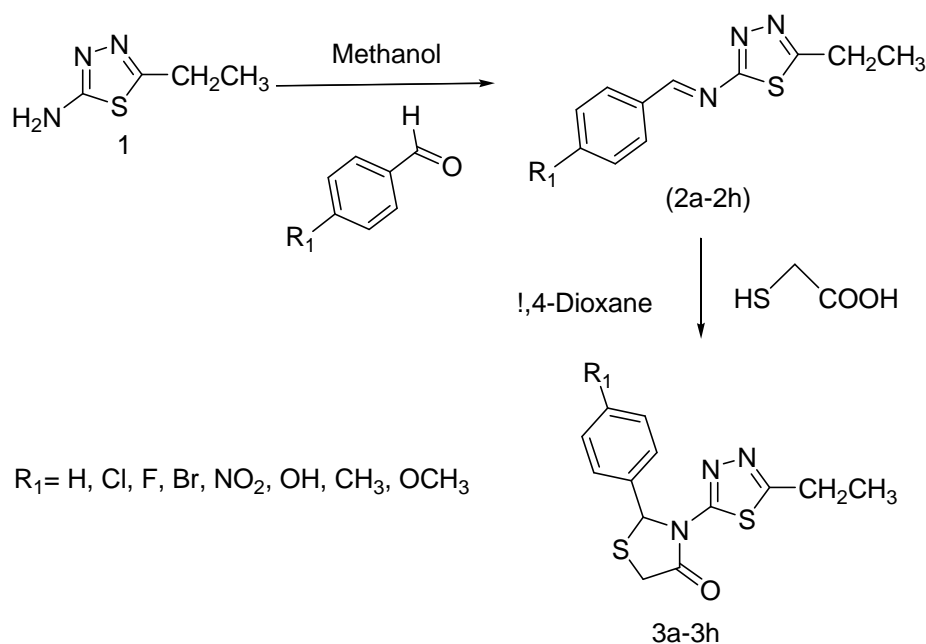
Scheme: Synthesis of 2-( p -substituted benzylidene)-3-(5-ethyl-1, 3, 4-thiadiazol-2-yl) thiazolidin-4-one
