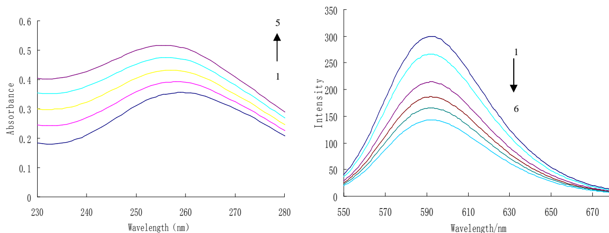
Figure 2. (a) Absorption Spectra of DNA-compound 8 in Tris-HCl Buffer Solution at pH 7.4. CT-DNA concentration was kept fixed at 10 mM and compound 10 concentration was varied from (1) 0 to (5) 20 mM; (b) Fluorescence emission spectra (excited at 520 nm) of EB, EB-DNA complexes in the absence (1) and presence (2-6) of increasing concentrations of the compound 8 (2 mmol L -1 , 1 L per scan)
