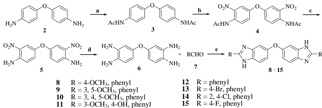
Scheme 2. Reagents and conditions: (a) (CH 3 CO) 2 O/NEt 3 , acetone, 0 °C, 2 h, 98%; (b) Conc. HNO 3 , acetic acid, 0-50 °C, 5 h, 98%; (c) 42% KOH aq, MeOH, reflux, 2 h, 97%; (d) Pd-C, H 2 , MeOH, rt, 6 h, 89%; (e) NaHSO 3 , methanol, rt, 8 h, 54-93%
