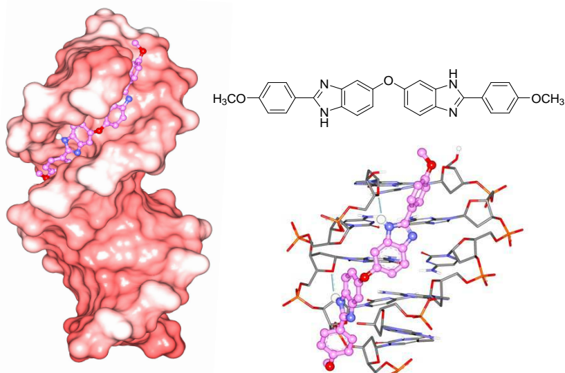
Figure 1. Close-up view of compound 8 binding in the minor groove
