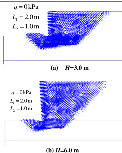
Fig. 13: Total incremental displacements of filling
