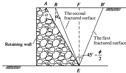
Fig. 4: Position of fractured surface of planar retaining wall
