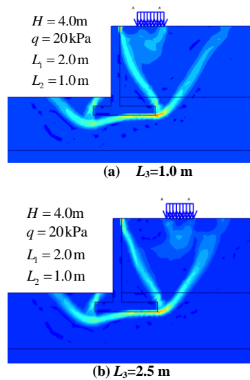
Fig. 10: Relationship between location of uniform load and position of fractured surface
