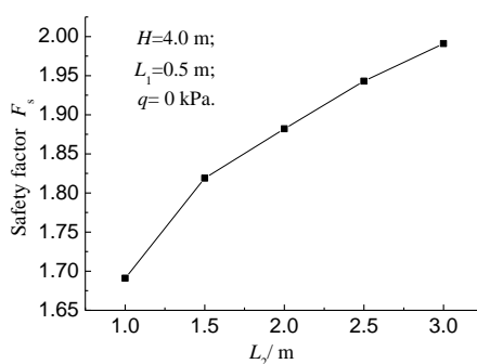
Fig. 9: Relationship between safety factor of retaining wall and width of toe plate
