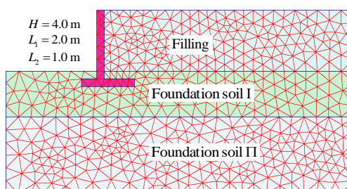
Fig. 2: Mesh of finite element method (elements: 1108)
