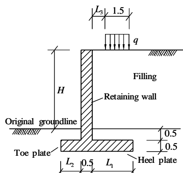
Fig. 1: Model of cantilever retaining wall (unit: m)
