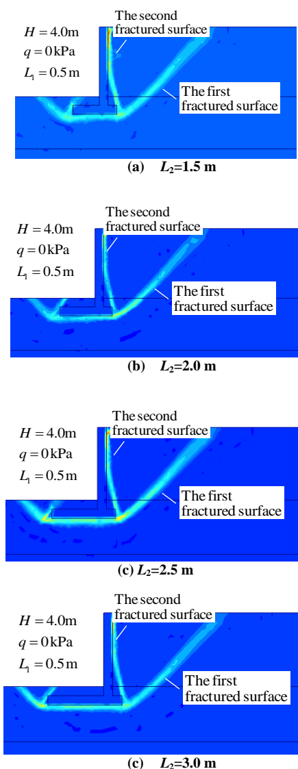
Fig. 8: Relationship between width of toe plate and position of fractured surface
