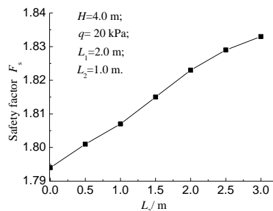
Fig. 11: Relationship between safety factor of retaining wall and location of uniform load
