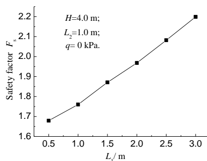
Fig. 7: Relationship between safety factor of retaining wall and width of heel plate
