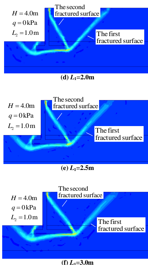
Fig. 3: Relationship between width of heel plate and position of fractured surface
