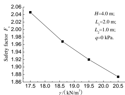
Fig. 15: Influence of gravity of filling on stability of retaining wall
