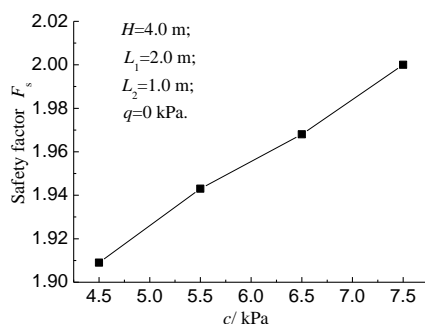
Fig. 16: Influence of cohesive strength of filling on stability of retaining wall
