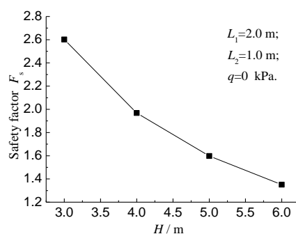
Fig. 14: Relationship between safety factor of retaining wall and its height
