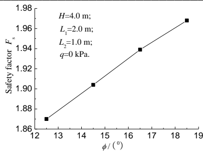
Fig. 17: Influence of internal friction angle of filling on stability of retaining wall
