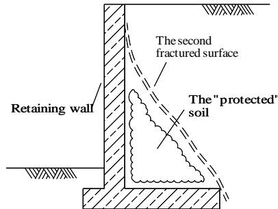
Fig. 5: Part of filling apart from fractured surface in cantilever retaining wall
