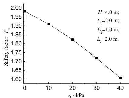
Fig. 12: Relationship between safety factor of retaining wall and value of uniform load
