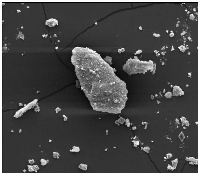
Figure 3: SEM image of particle of cobalt(II) complex
