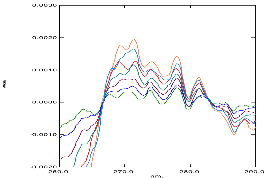
Fig. 1(b): Overlay spectra of second order derivative of thiocolchicoside in the concentration range of 2 and 14 \mu\text{g/ml} at 278.2 nm
