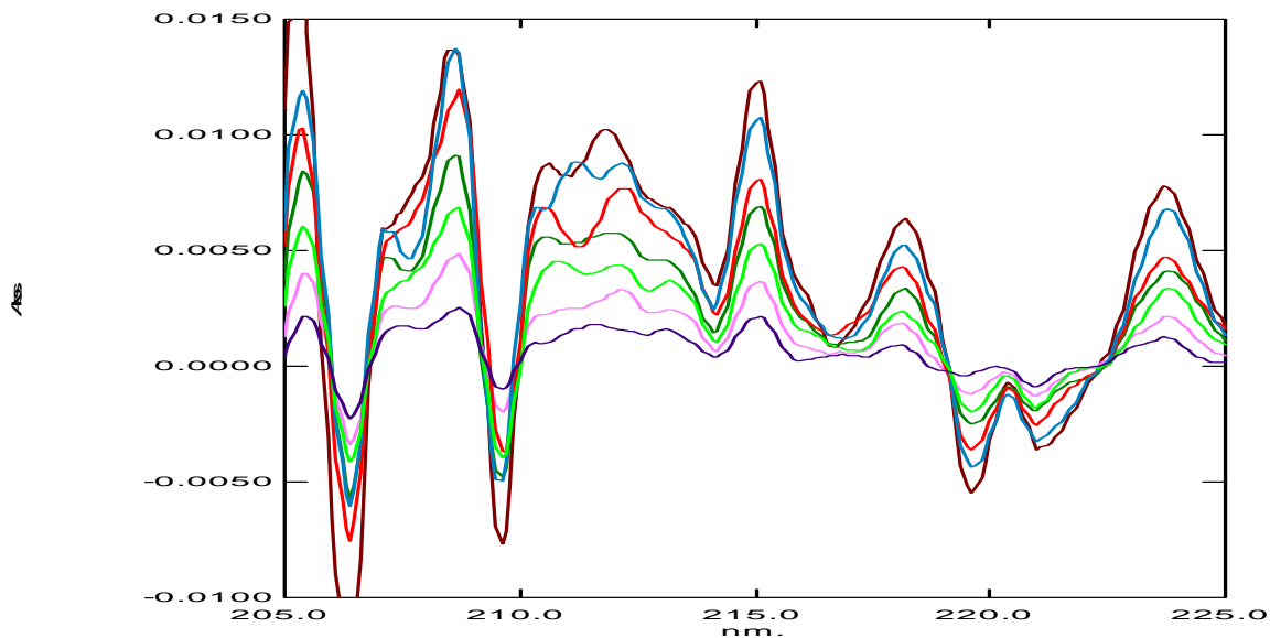
Fig. 1(b): Overlay spectra of second order derivative of thiocolchicoside in the concentration range of 2 and 14 \mu\text{g/ml} at 278.2 nm
