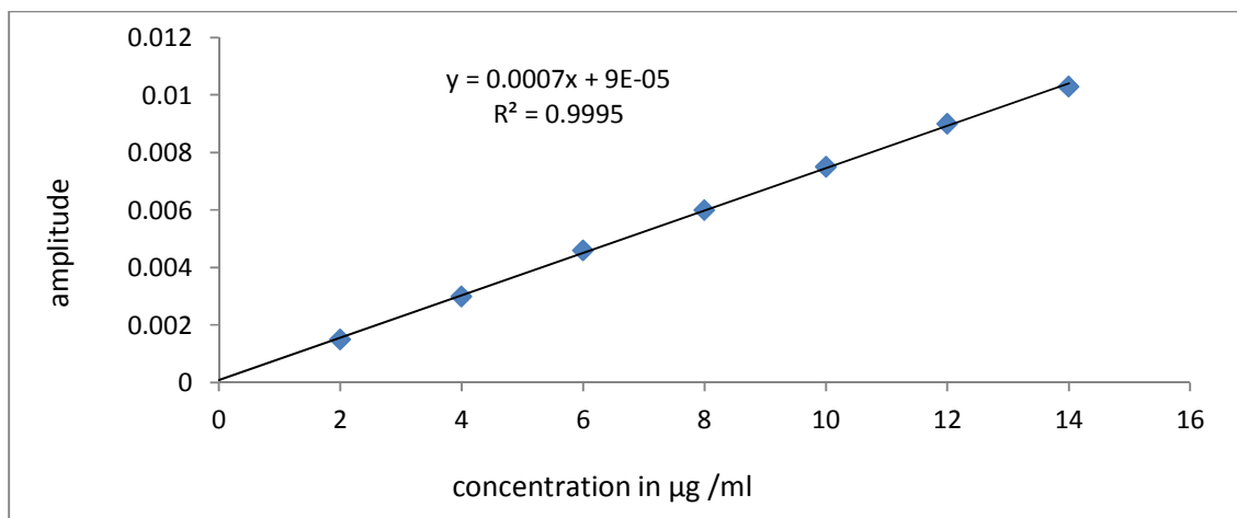
Fig.2 (b): Calibration curve of thicolchicoside in the concentration range of 2-14 µg/ml
