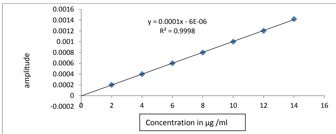
Fig.2 (b): Calibration curve of thicolchicoside in the concentration range of 2-14 µg/ml
