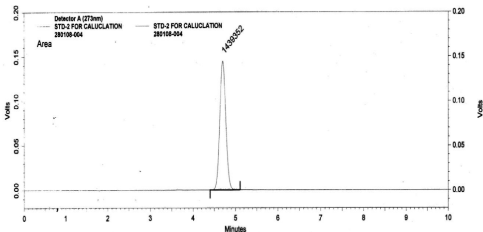
Figure 2 Chromatogram of Standard solution of Valsartan
