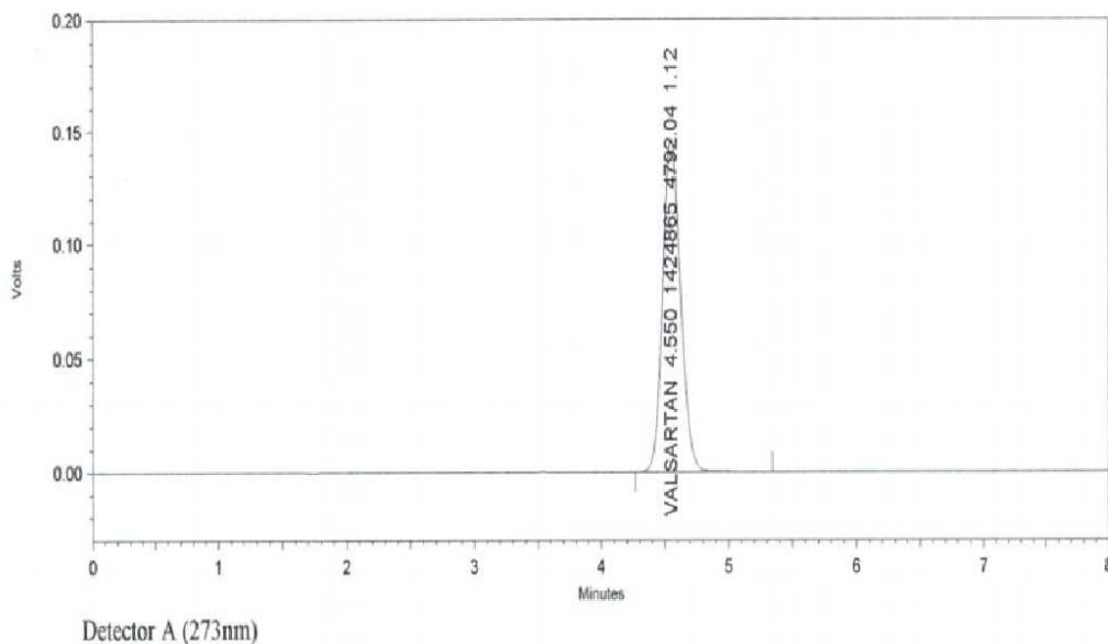
Figure 3 Chromatogram of Test solution of Valsartan
