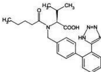
Fig 1: Structure of valsartan
