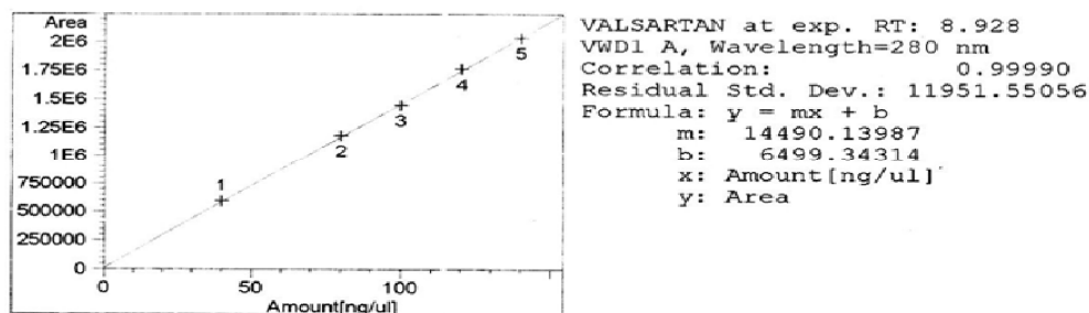
Figure 4 Linear calibration curve for Valsartan
