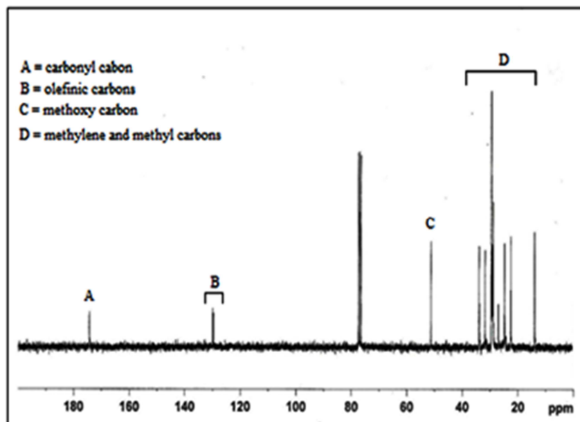
Fig. 4. ^{13}\text{C} NMR spectrum of FAME from Abelmoschus esculentus seed oil
