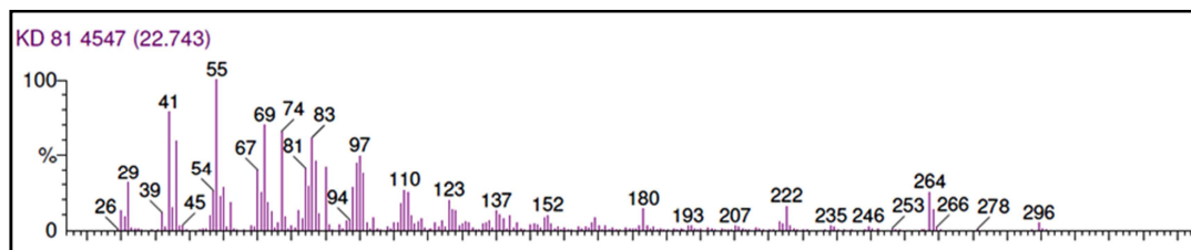
Fig. 2c. Mass spectrum of methyl oleate
