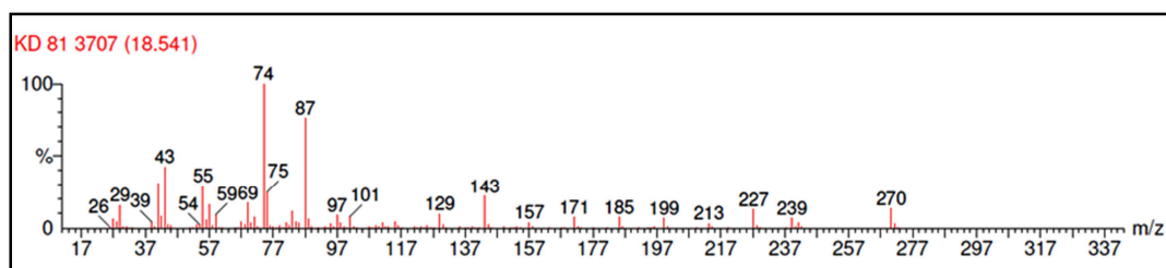
Fig. 2a. Mass spectrum of methyl palmitate
