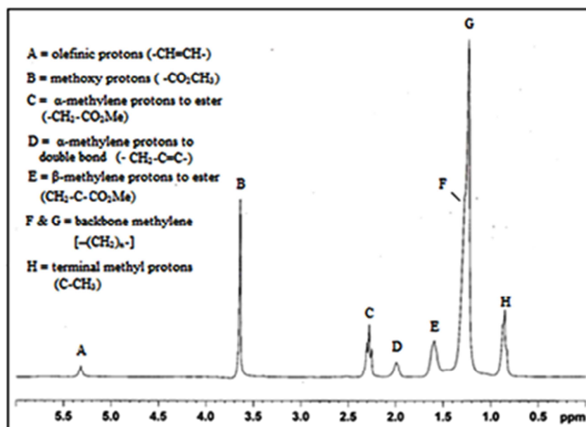
Fig. 3. ^1\text{H} NMR spectrum of FAME from Abelmoschus esculentus seed oil
