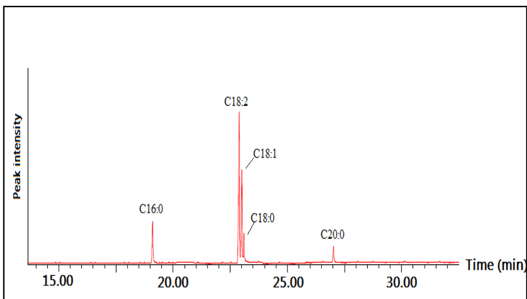
Fig. 2. Gas Chromatogram of FAME from Abelmoschus esculentus seed oil
