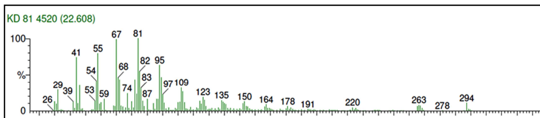
Fig. 2b. Mass spectrum of methyl linoleate
