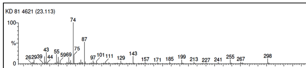
Fig. 2d. Mass spectrum of methyl stearate
