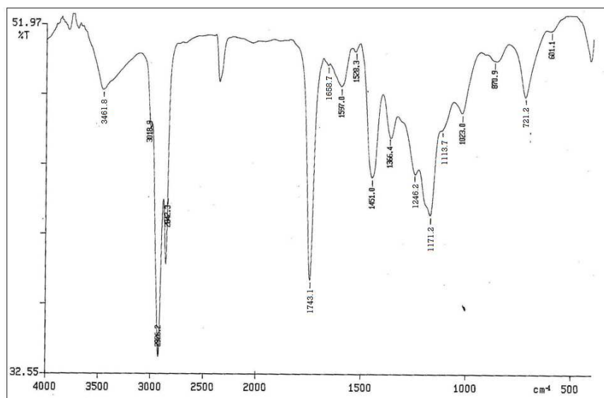
Fig 5. The IR spectrum of FAME from Abelmoschus esculentus seed oil
