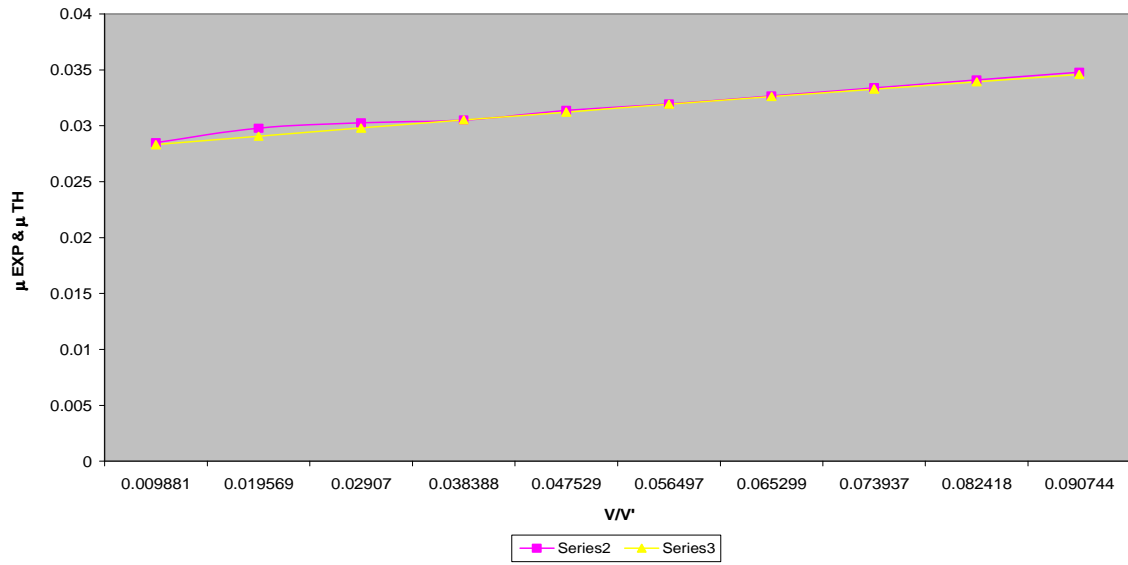
Fig 2 GRAPH FOR LINEAR ATTENUATION COEFFICIENT FOR ANILINE SOLUTION IN ETHANOL FOR ENERGY 0.36 MeV
