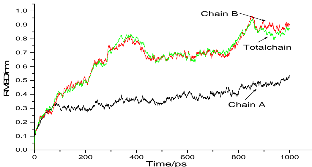
Figure 1: Plot of root mean square deviation (RMSD) with simulation time
