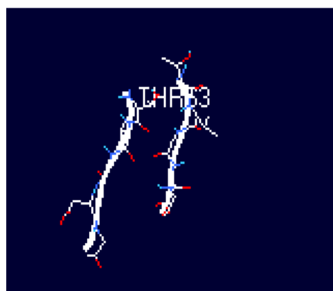
Figure 6b.Snapshot at 308ps
