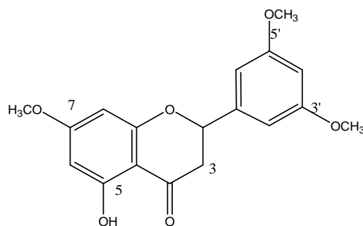
Figure 2. Structure of the isolated compound from Aglaia odorata L (3',5', 7 tri-O-metil Naringenin)
