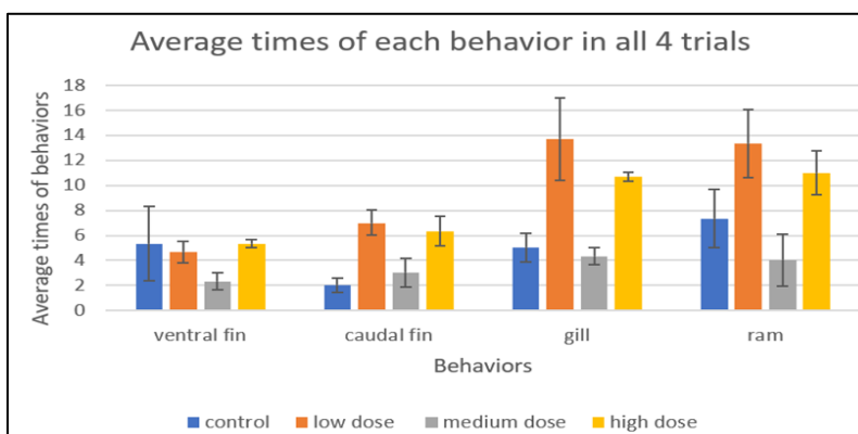
Figure 4: Average times of each behaviour in all 4 trials
