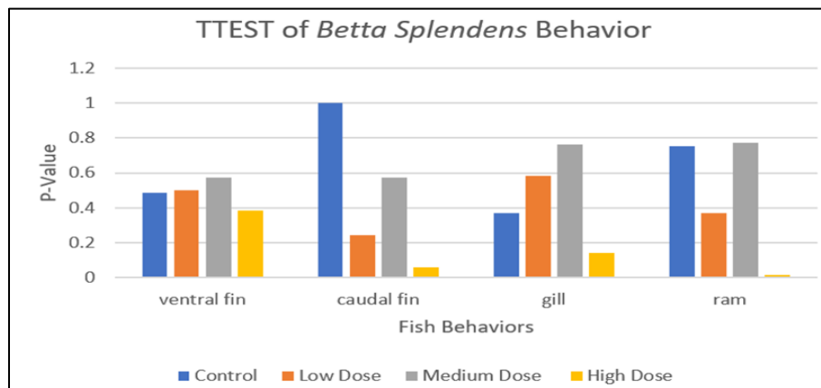
Figure 3: T-Test on the behaviour of fish in different doses of caffeine
