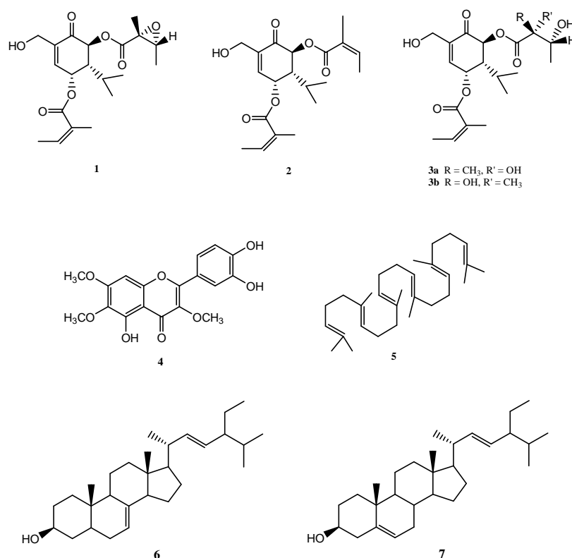
Fig. 1. Chemical constituents of Sphaeranthus africanus : carvotanacetone derivatives (1-3b), chrysofenol D (4), squalene (5), spinasterol (6), and stigmasterol (7)
